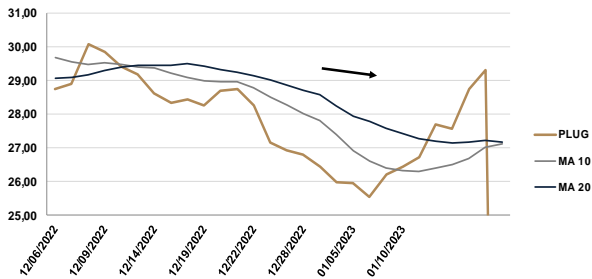
Figure 1: The Main Graph shows the down stock's trend.
