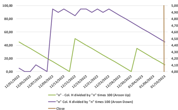
Figure 4: Aroon Indicator indicates a sell signal
