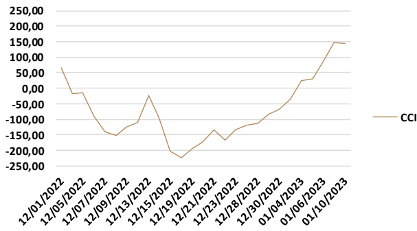
Figure 2: CCI indicates an ambiguous sell signal.
