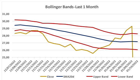
Figure 3: Bollinger Band indicates a buy signal.
