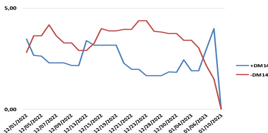
Figure 5: DMI shows a sell signal
